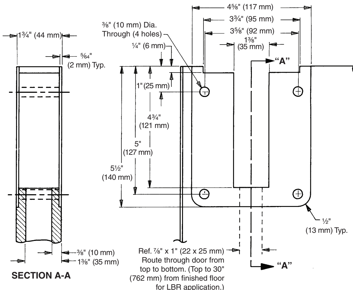
RELEASE PLUNGER DETAIL
