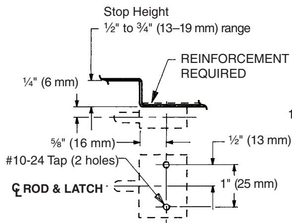
RELEASE PLUNGER DETAIL
